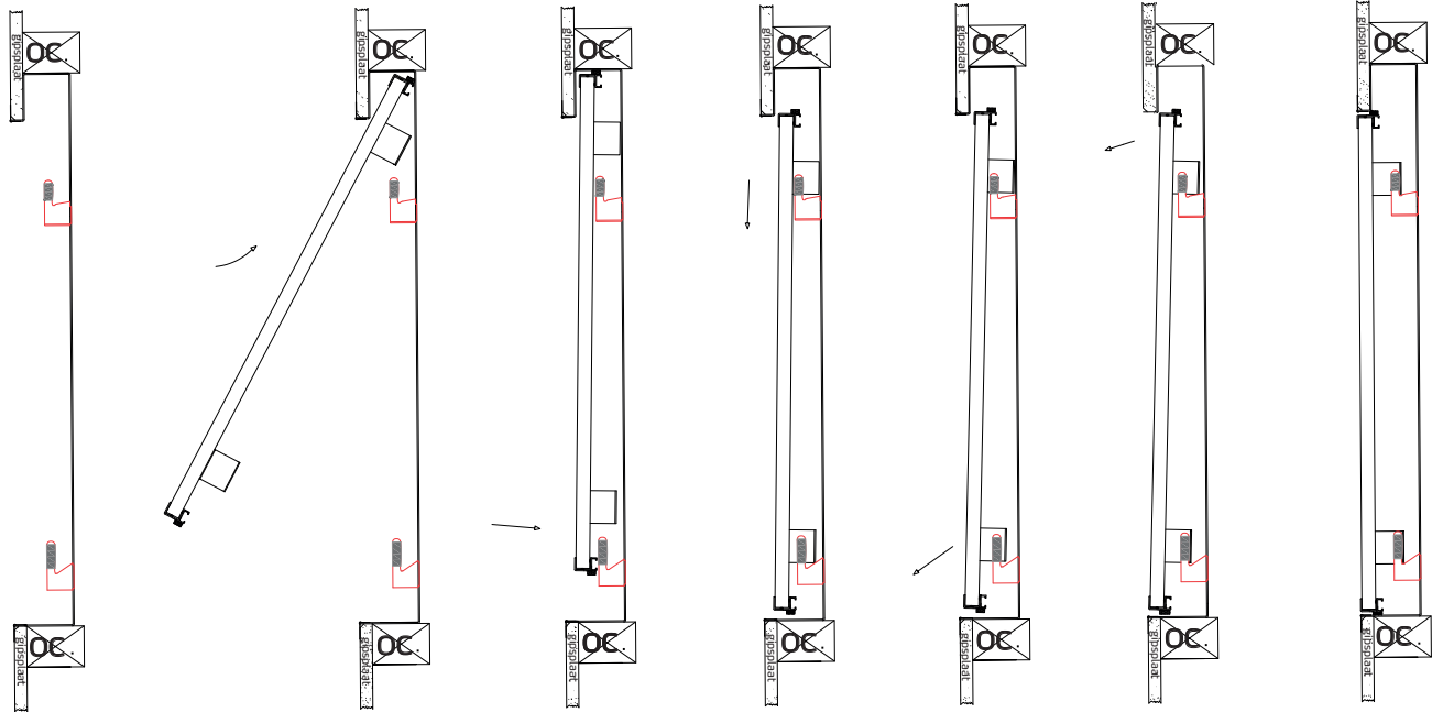
Wandmontage
